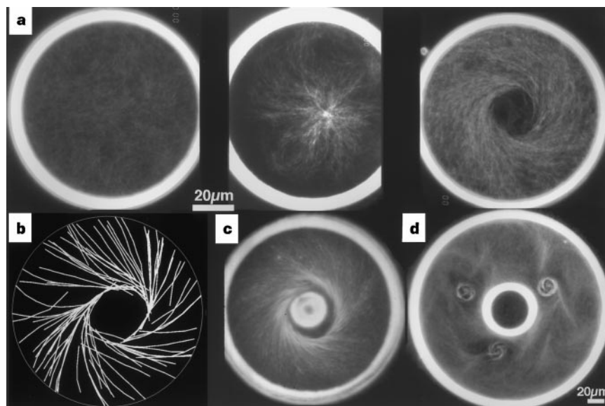
Figure 2 Self-organization in the constrained geometry of micro-fabricated chambers etched in glass. a , Formation of a vortex as observed by dark-field microscopy in a chamber of diameter 90 \mu\text{m} and depth 5 \mu\text{m} . Microtubule polymerization has been initiated by warming to 37°C. Left, after ~0.5 min, microtubules nucleate uniformly in the sample; middle; after ~1.5 min, an aster forms in the centre of the chamber; right, after ~3 min, a steady-state vortex structure is observed. b , Two-dimensional numerical simulation of the same process. The microtubule mean length was initially smaller than the chamber radius, but became longer than it in the state shown. c , Vortex structure in a torus-shaped chamber of the same diameter as previously, but including a central unetched region. d , Steady-state structure in a torus-shaped chamber of larger size (240 \mu\text{m} ). The three vortices have the same core size as those in a and c . Scale bars, 20 \mu\text{m} .
